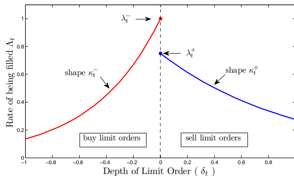
Figure 3: Fill rates \Lambda_t^\pm with \kappa_t^+ = 2 , \kappa_t^- = 1 , \lambda_t^+ = 0.75 and \lambda_t^- = 1 . As \kappa_t^\pm evolve, the fill rate shape changes, while the MO activity rates \lambda_t^\pm modulate the vertical scale. The maximum fill rate is achieved at \delta = 0 .
