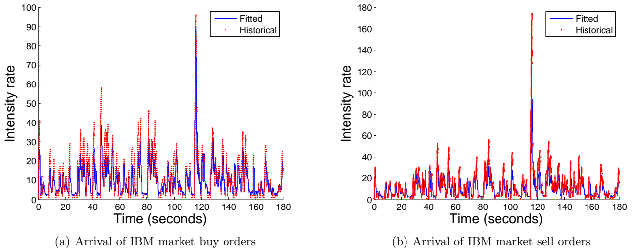
Figure 1: IBM MOs. Historical running intensity versus smoothed fitted intensity (restricted to \rho = 1 ) using a 1 second sliding window for IBM for a 3 minute period, between 3.30 and 3.33 pm, February 1 2008.
